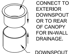
Downspout Stub Size: Std. 3" Dia.
