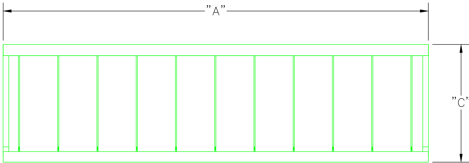
LFS - TR (WITHOUT BOX) FRONT VIEW WITH STANDING SEAM
