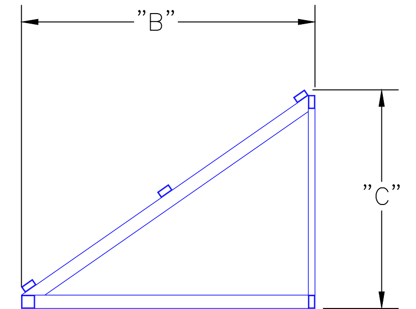
LFS - TR (WITHOUT BOX) SIDE VIEW - FRAME ONLY
