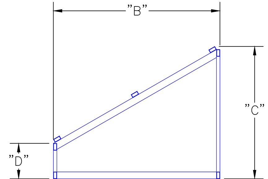
LFS - TR (WITH BOX) SIDE VIEW - FRAME ONLY
