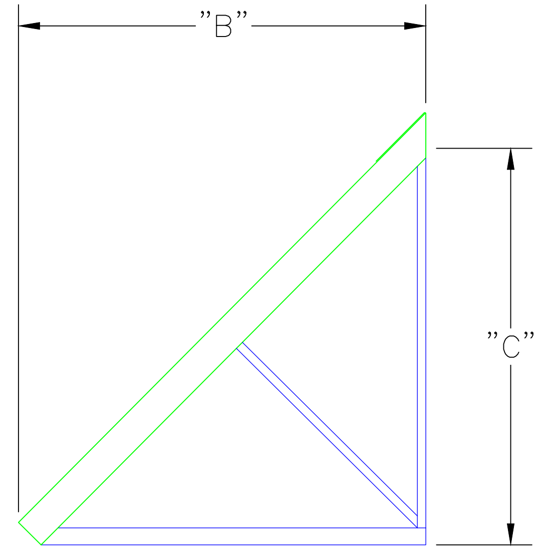
LFS - SLP SIDE VIEW WITH STANDING SEAM
