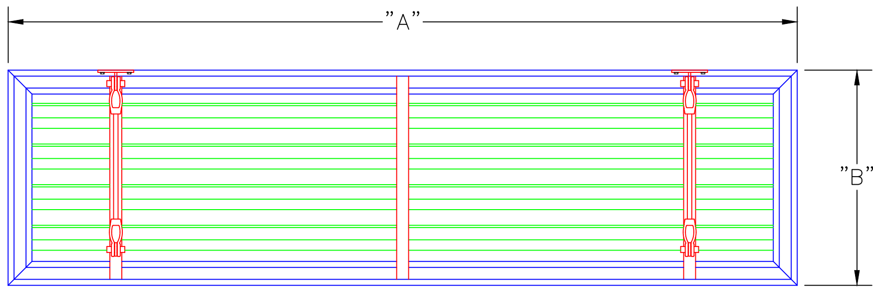
LFS - FLV PLAN VIEW
