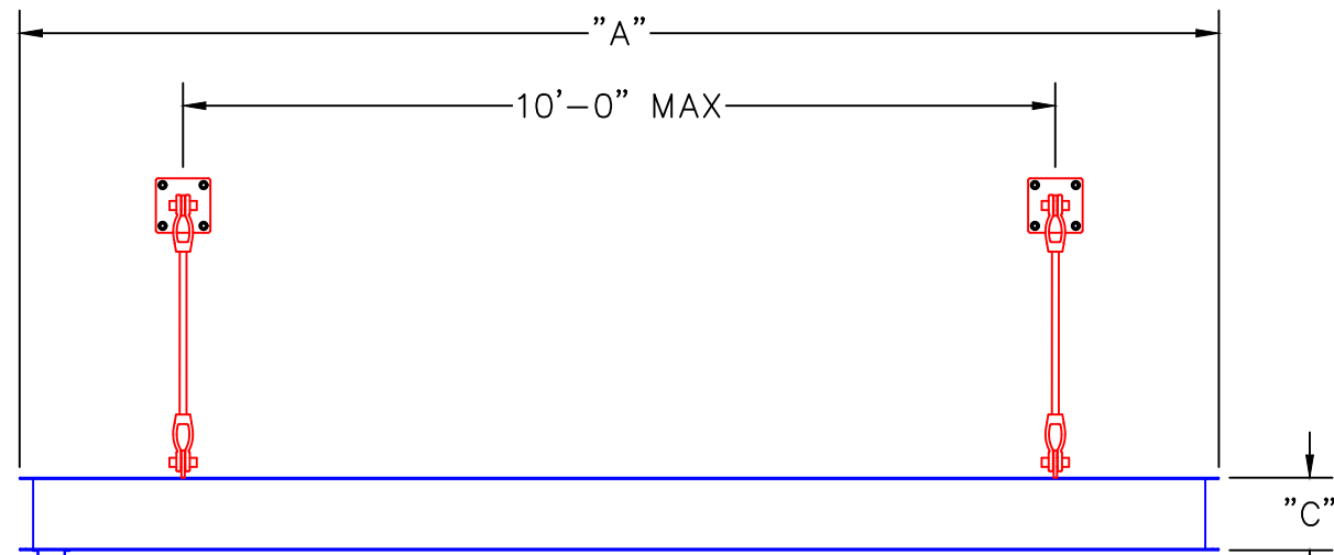
LFS - FLCA FRONT VIEW
