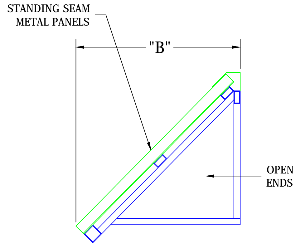
SIDE VIEW
