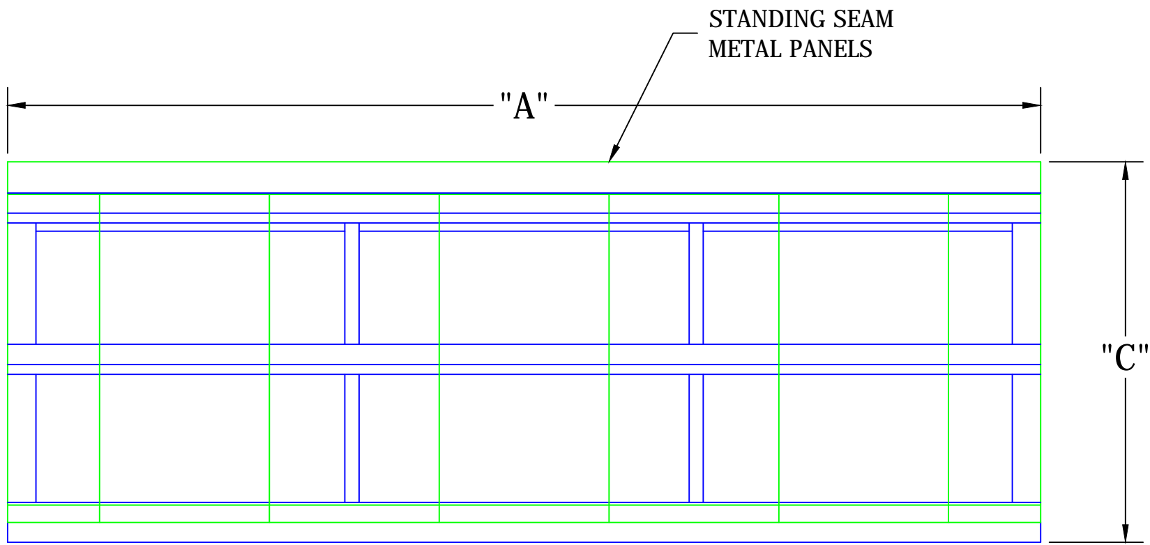
FRONT VIEW
