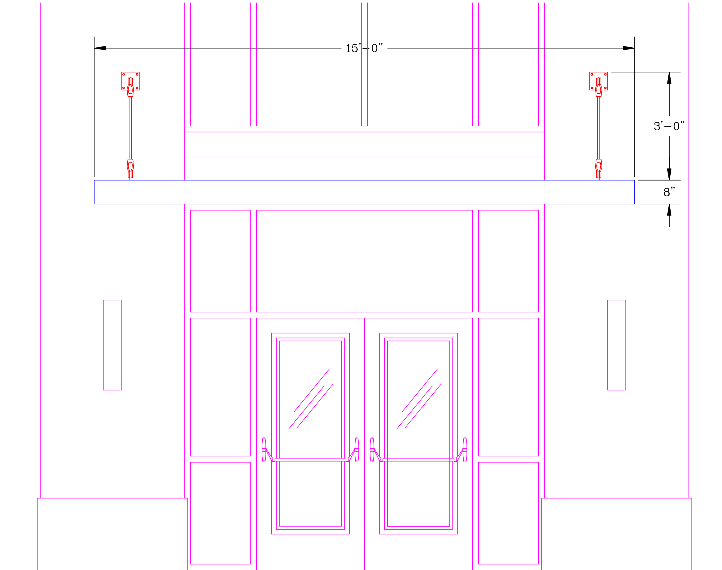
FRONT ELEVATION
